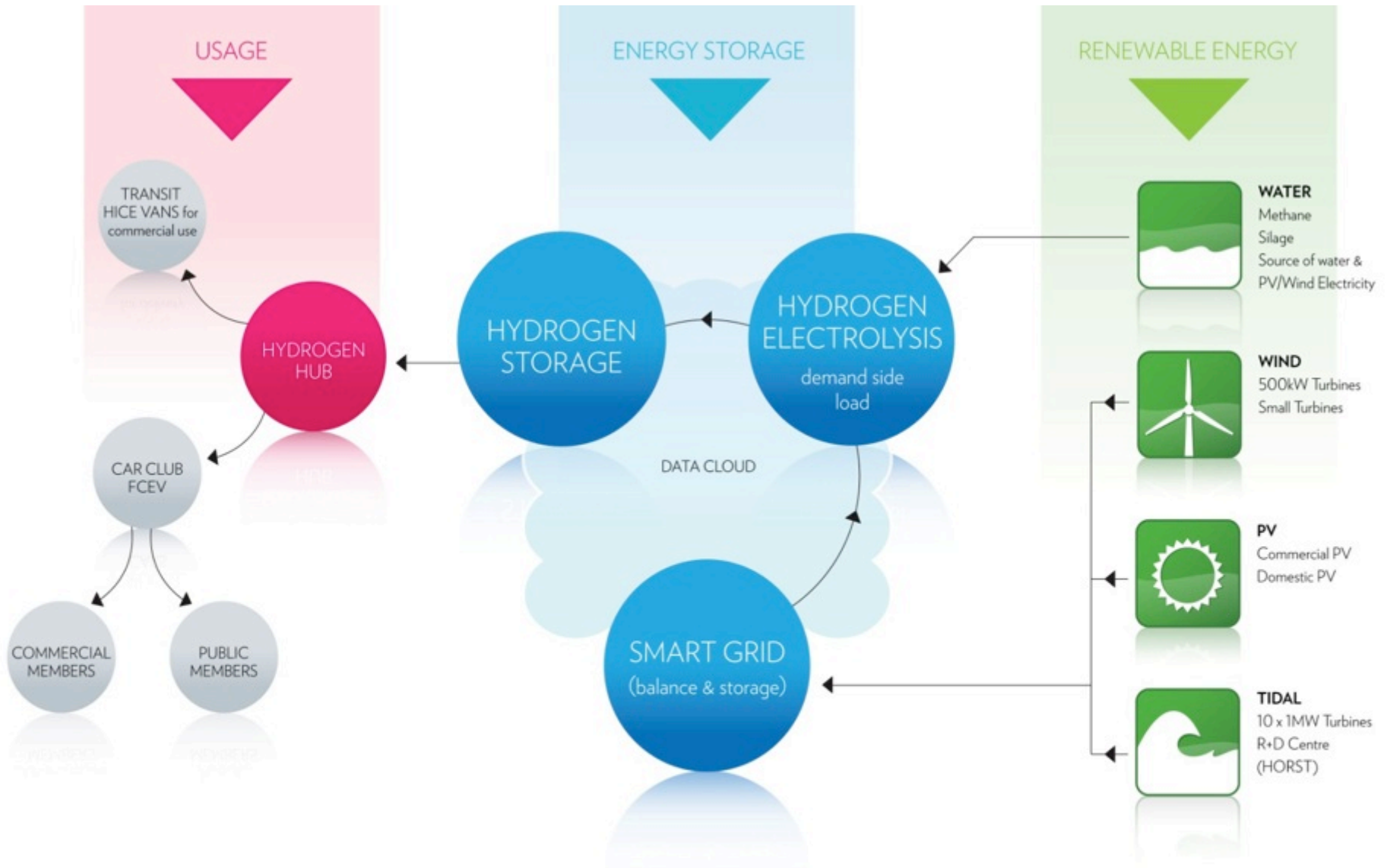
HYDROGEN SMART GRID INTEGRATION Energy Storage / Clean Fuel
